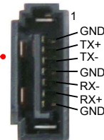
SATA_1/2/3/4/5/6
